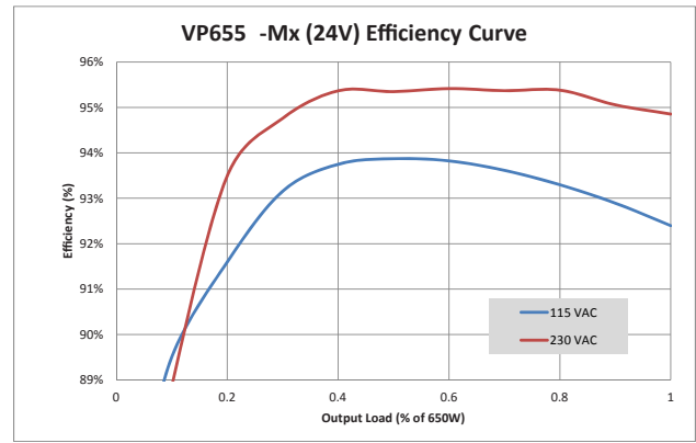
Figure 4. Typical Efficiency for 24 V Output
